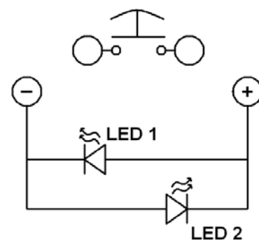
SPST with dual LED
